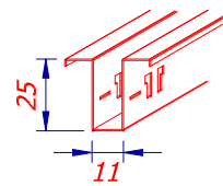
PRINCIPAL SPACIAL TILE
